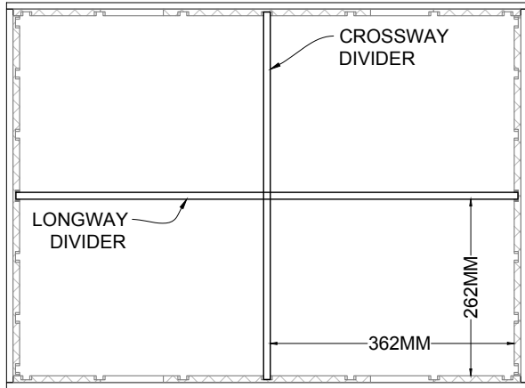
FOUR POCKET CONFIGURATION
