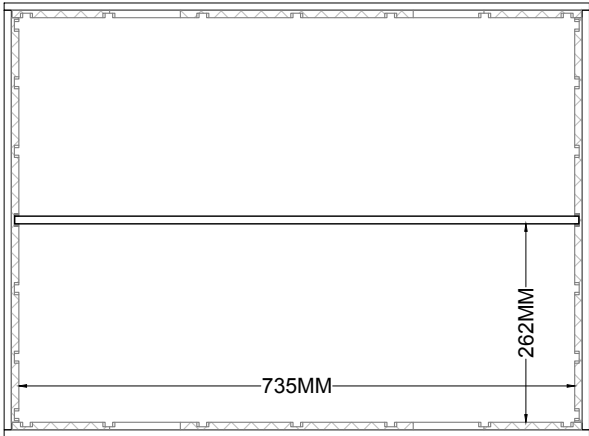
TWO POCKET CONFIGURATION
